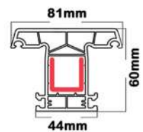
Fixed middle profile
