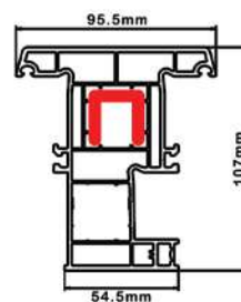
Monorail mulion
