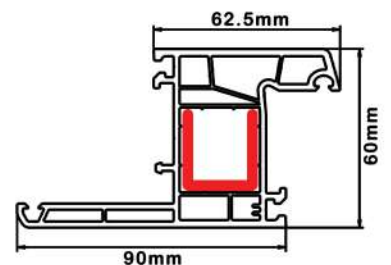
Renovation frame
