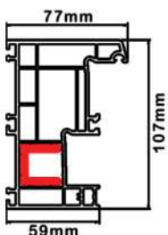
Single rail profile
