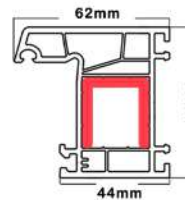
Frame profile
