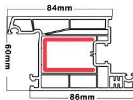
Door opening profile
